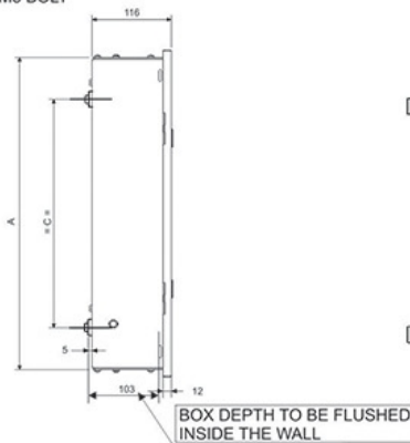
MOUNTING HOLE SUITABLE FOR M8 BOLT
