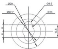
MOUNTING HOLE DETAILS SUITABLE FOR M12 BOLT
