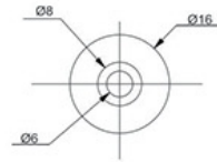
MOUNTING HOLE DETAILS SUITABLE FOR M5 BOLT
