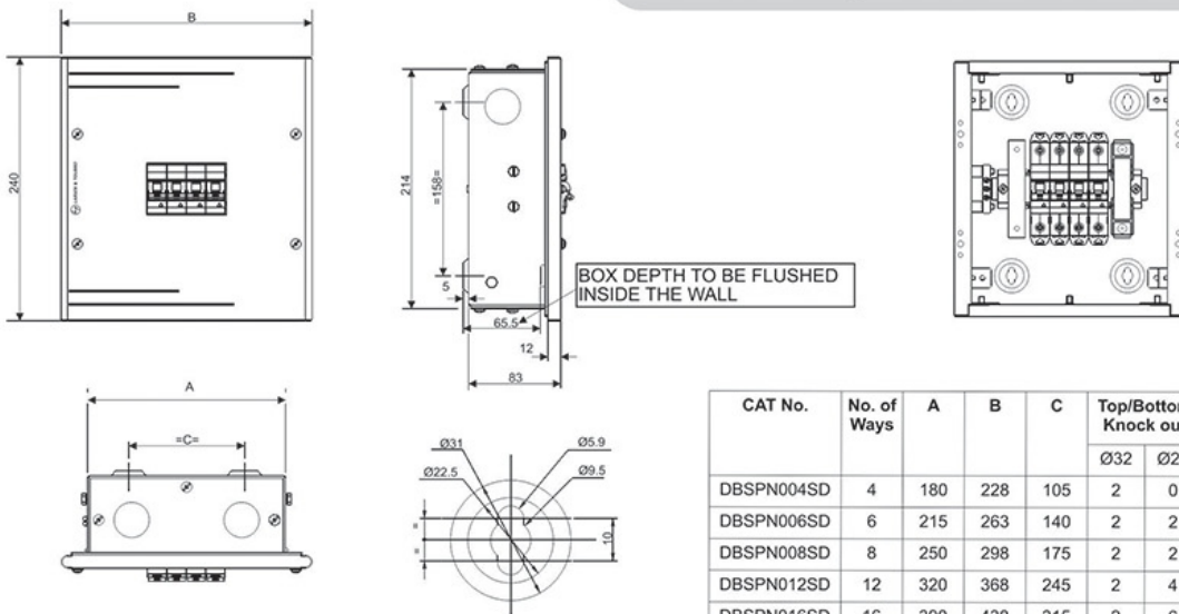
MOUNTING HOLE DETAILS SUITABLE FOR M8 BOLT
