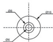
MOUNTING HOLE DETAILS SUITABLE FOR M5 BOLT
