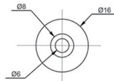
MOUNTING HOLE DETAILS SUITABLE FOR M5 BOLT
