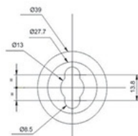
MOUNTING HOLE DETAILS SUITABLE FOR M12 BOLT
