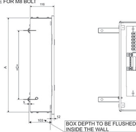
MOUNTING HOLE SUITABLE FOR M8 BOLT
