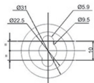
MOUNTING HOLE DETAILS SUITABLE FOR M8 BOLT
