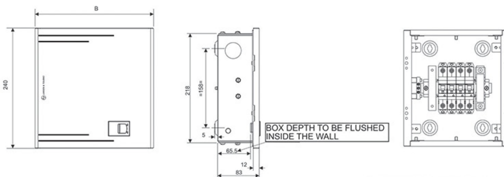
MOUNTING HOLE DETAILS SUITABLE FOR M8 BOLT
